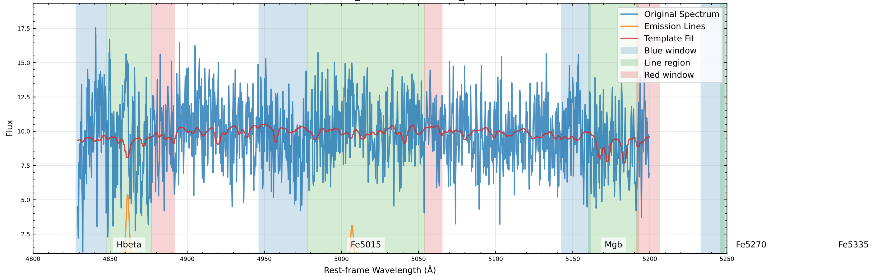
Original Data Comparison (v_star=-201.6 km/s, v_gas=-65.4 km/s)
