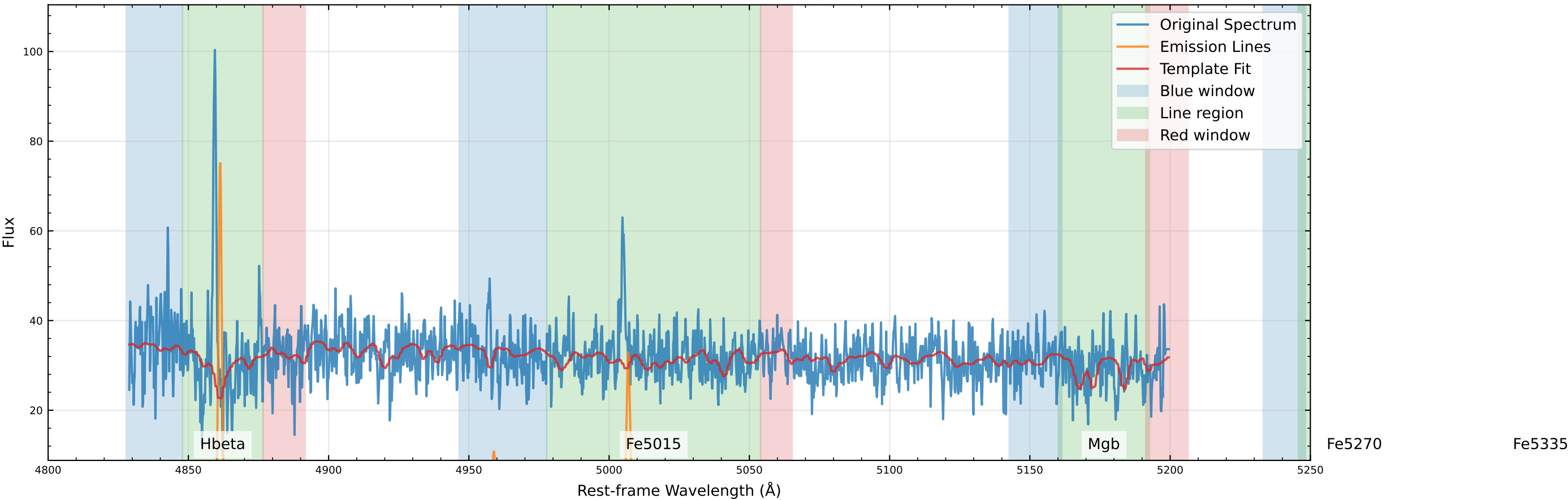
Original Data Comparison (v_star=-128.7 km/s, v_gas=-119.2 km/s)
