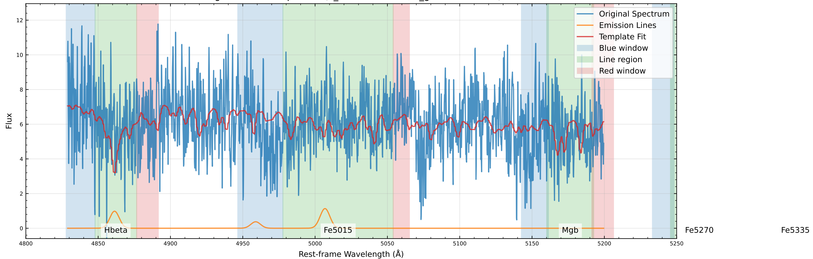
Original Data Comparison (v_star=-6.6 km/s, v_gas=-25.2 km/s)
