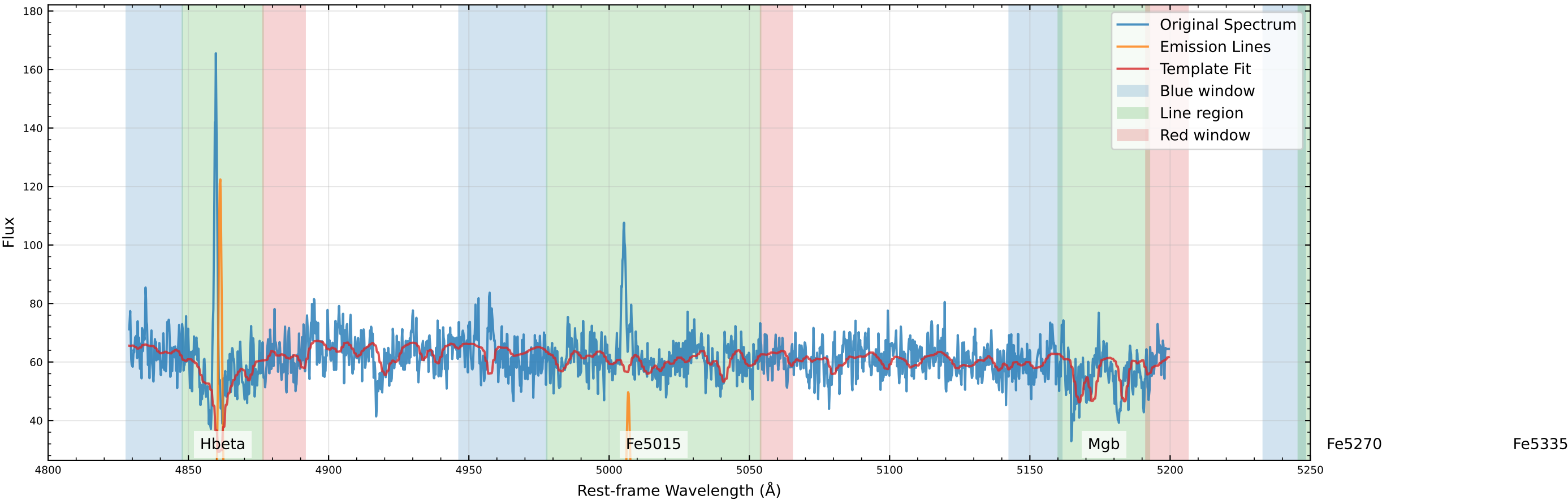
Original Data Comparison (v_star=-110.3 km/s, v_gas=-97.8 km/s)
