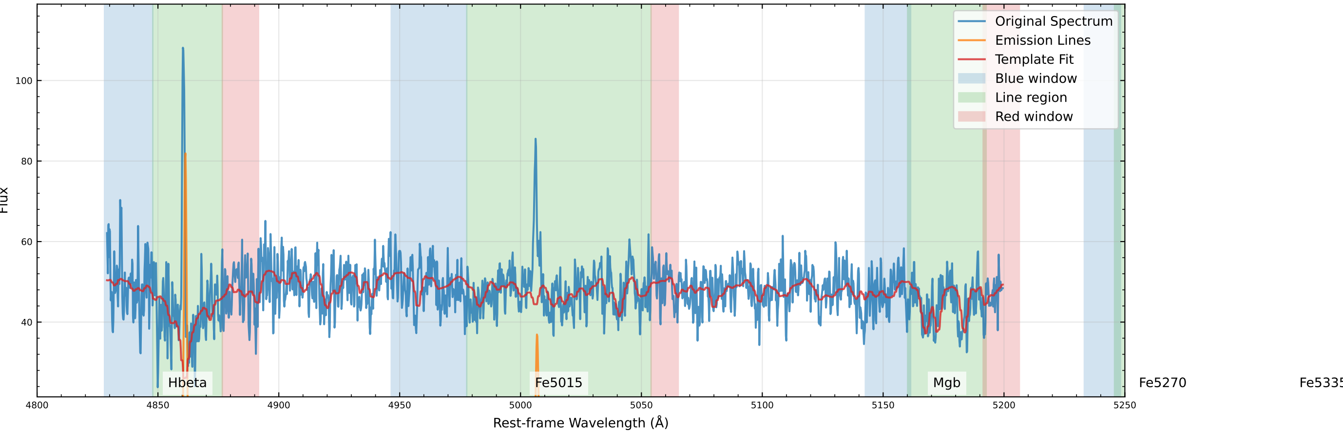
Original Data Comparison (v_star=-58.0 km/s, v_gas=-50.3 km/s)
