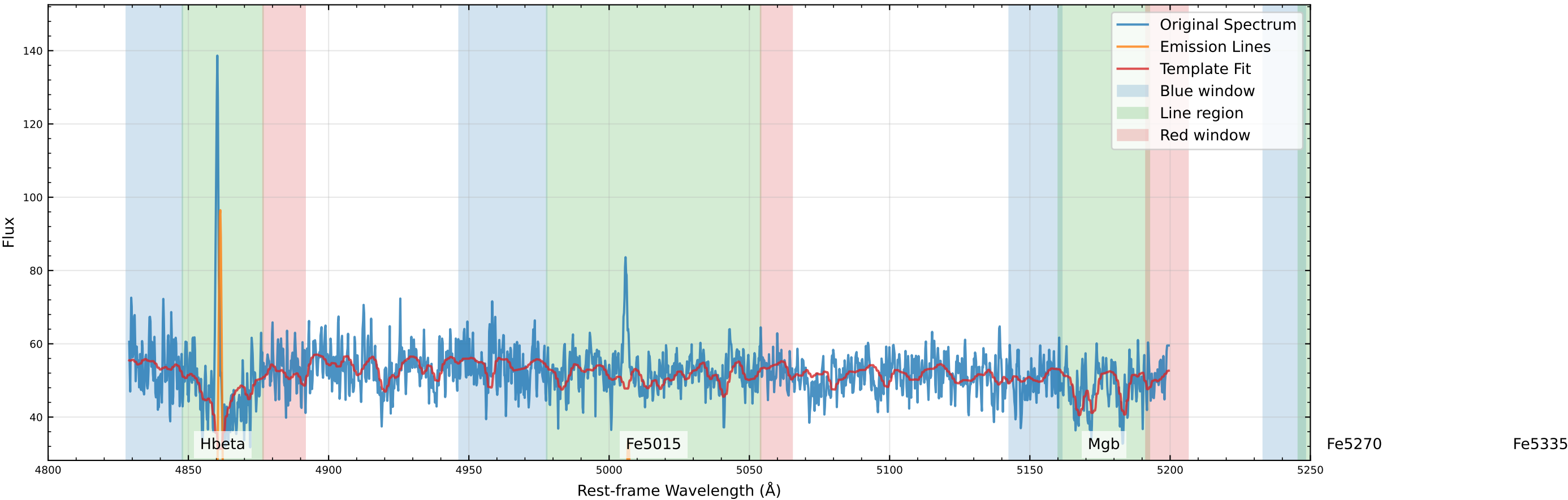
Original Data Comparison (v_star=-72.0 km/s, v_gas=-63.7 km/s)
