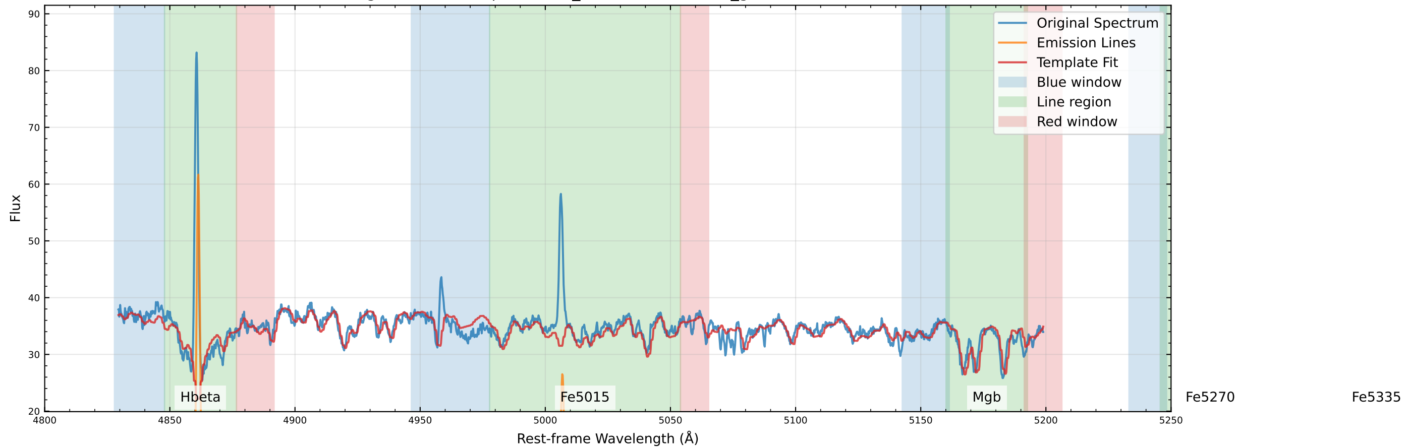
Original Data Comparison (v_star=-42.6 km/s, v_gas=-41.4 km/s)
