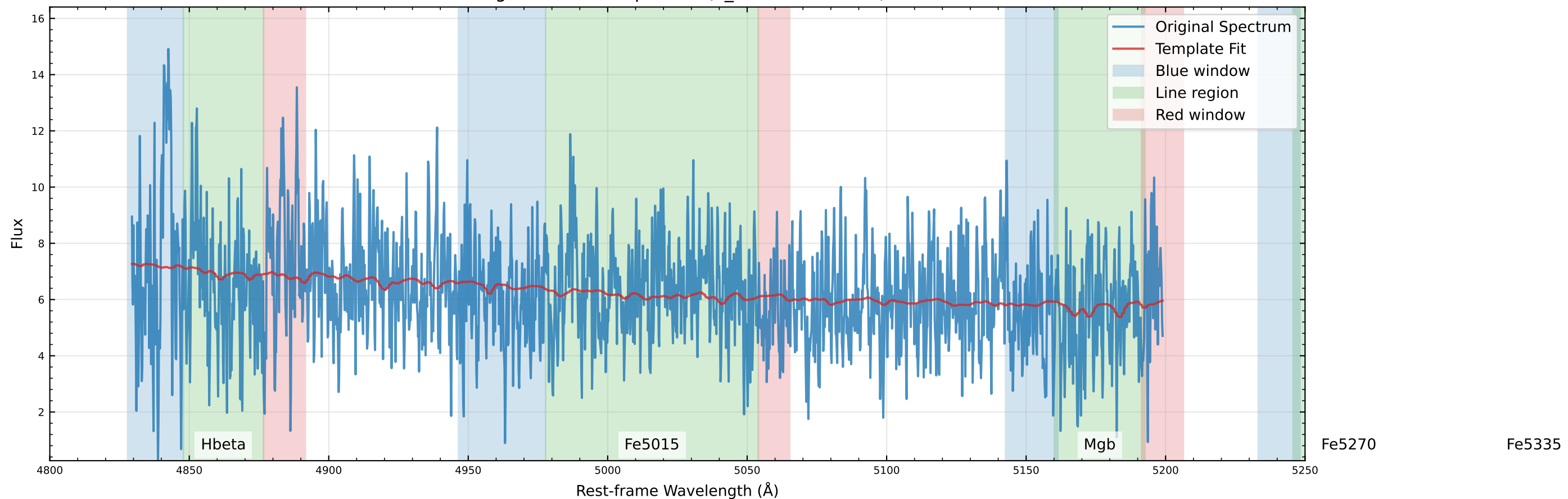
Original Data Comparison (v_star=-78.0 km/s)
