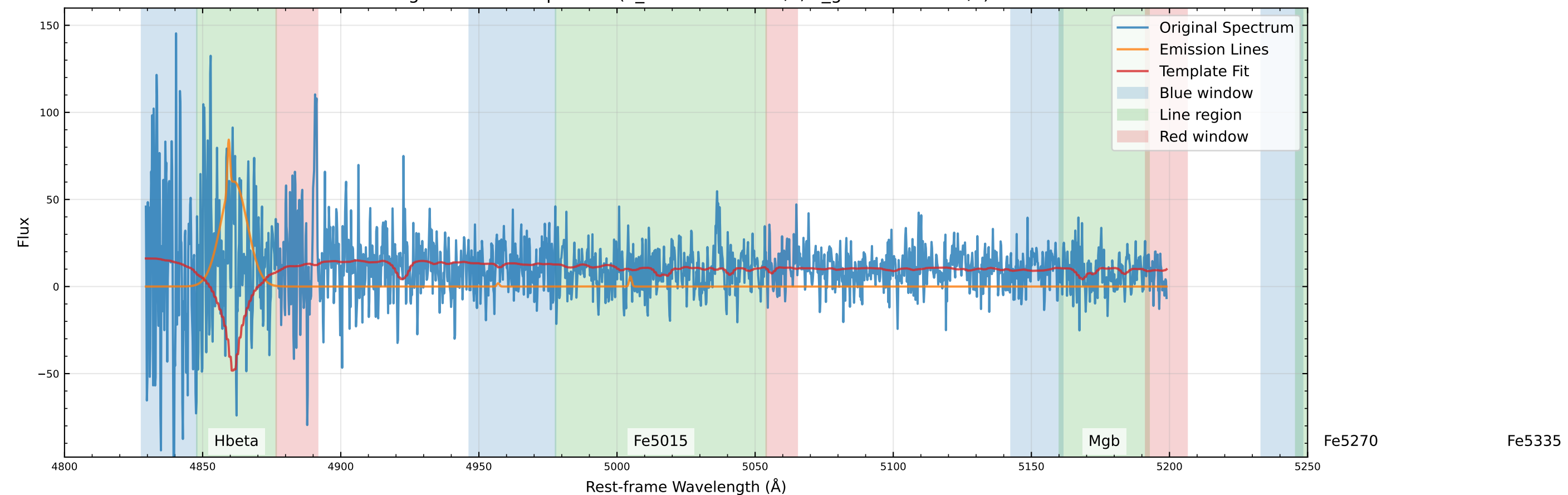
Original Data Comparison ( v_{\text{star}}=-416.9 km/s, v_{\text{gas}}=-253.3 km/s)
