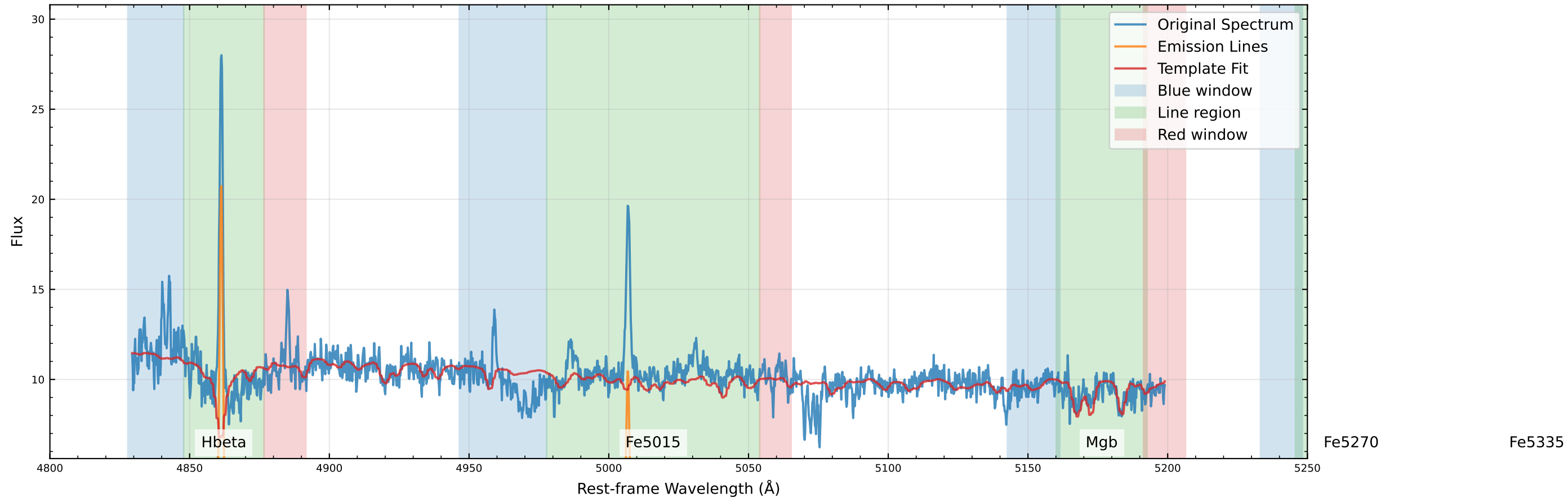
Original Data Comparison (v_star=-31.3 km/s, v_gas=1.1 km/s)
