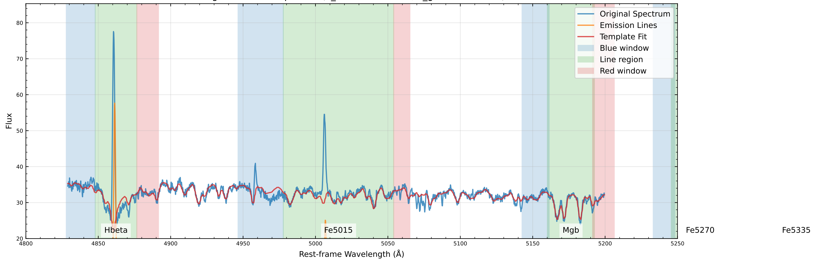
Original Data Comparison (v_star=-42.5 km/s, v_gas=-42.2 km/s)
