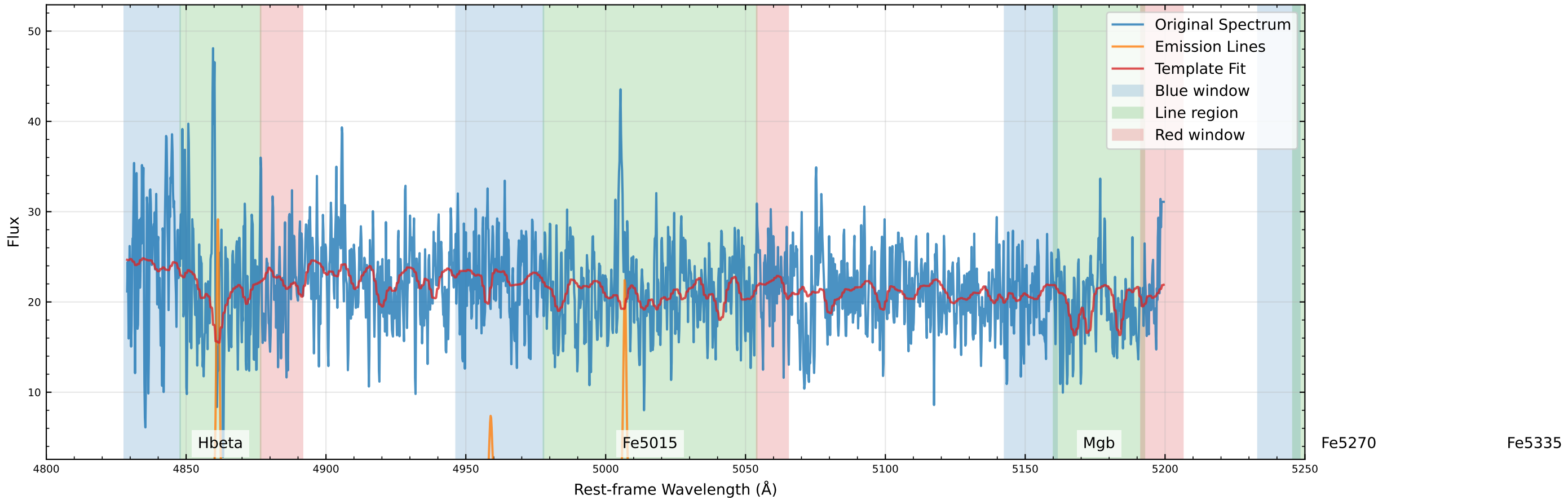
Original Data Comparison (v_star=-99.4 km/s, v_gas=-94.1 km/s)
