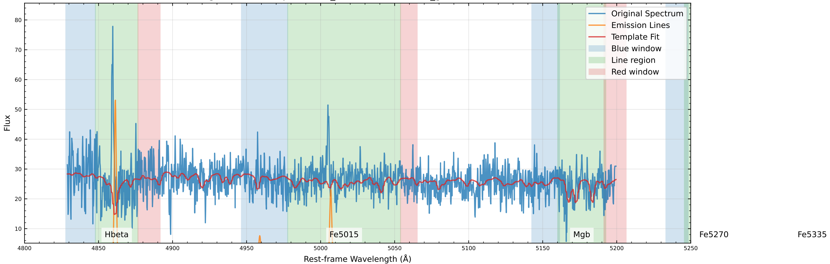
Original Data Comparison (v_star=-108.1 km/s, v_gas=-113.9 km/s)
