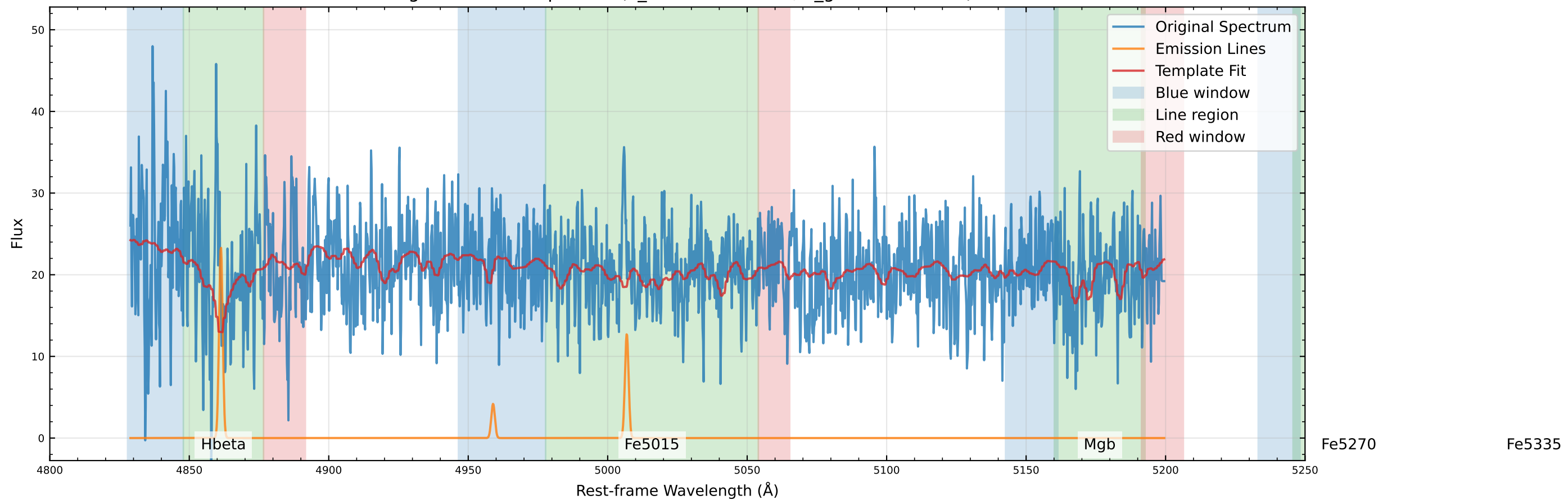
Original Data Comparison (v_star=-58.3 km/s, v_gas=-81.0 km/s)
