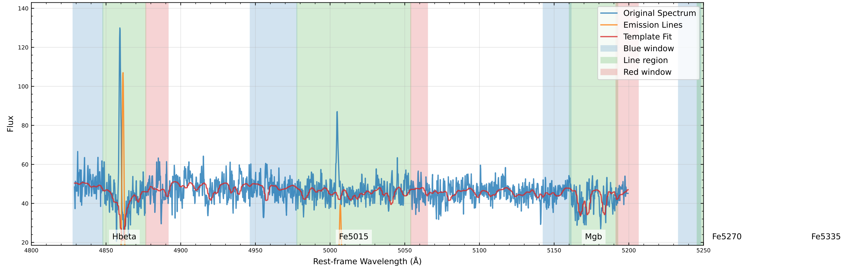
Original Data Comparison (v_star=-127.1 km/s, v_gas=-123.5 km/s)
