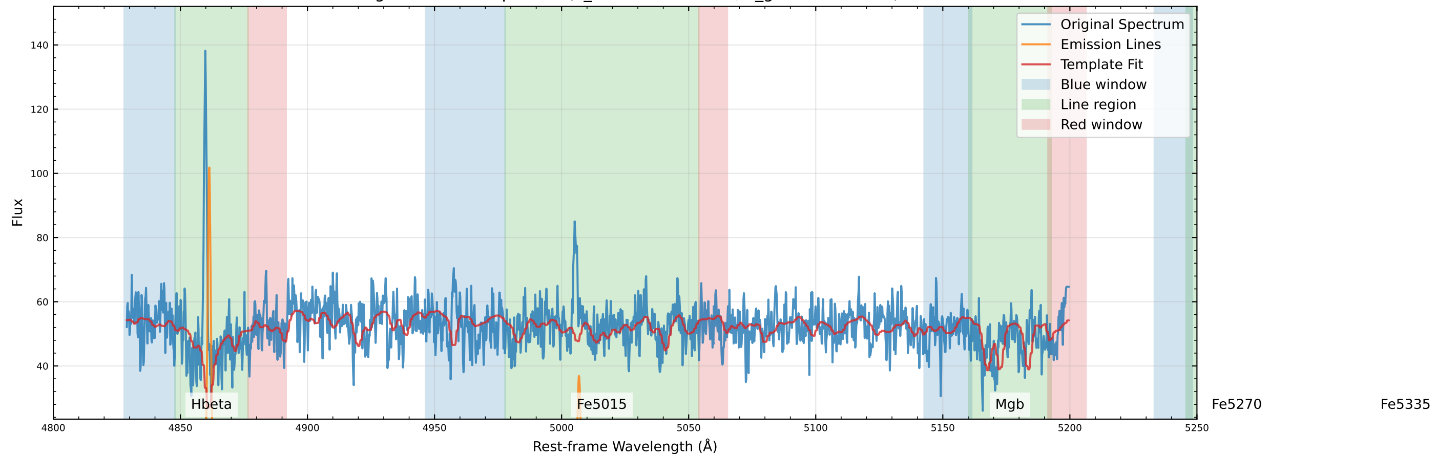
Original Data Comparison (v_star=-107.0 km/s, v_gas=-94.0 km/s)
