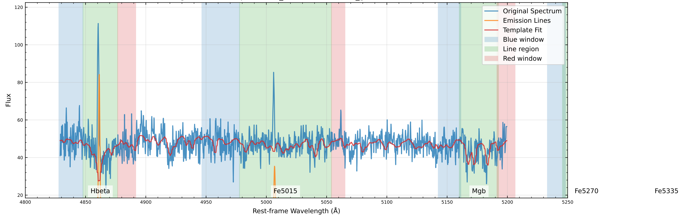
Original Data Comparison (v_star=-60.6 km/s, v_gas=-51.1 km/s)
