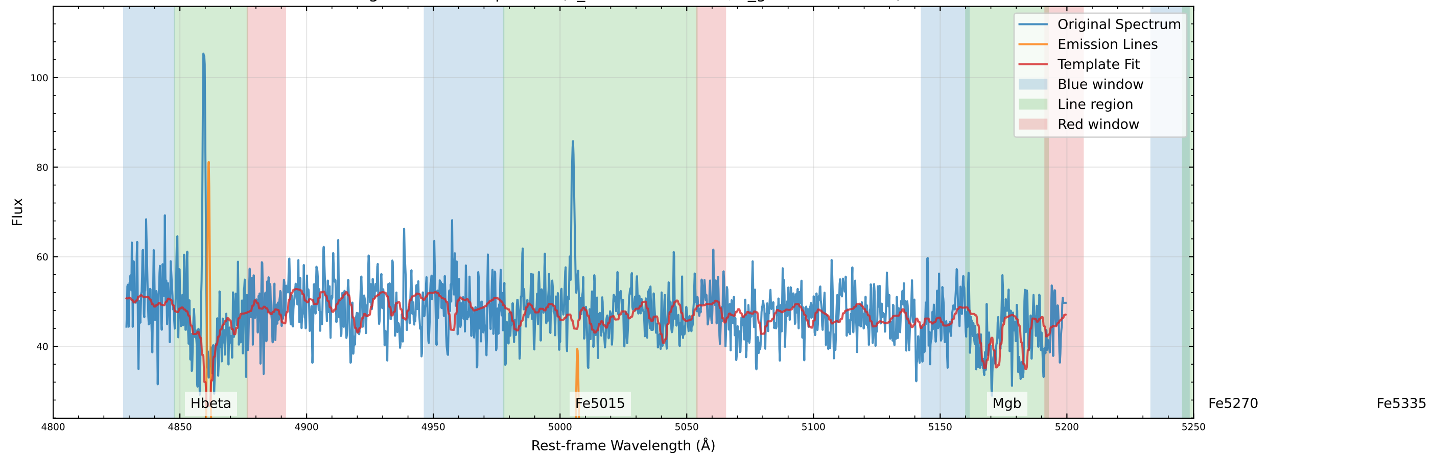
Original Data Comparison (v_star=-118.4 km/s, v_gas=-112.8 km/s)
