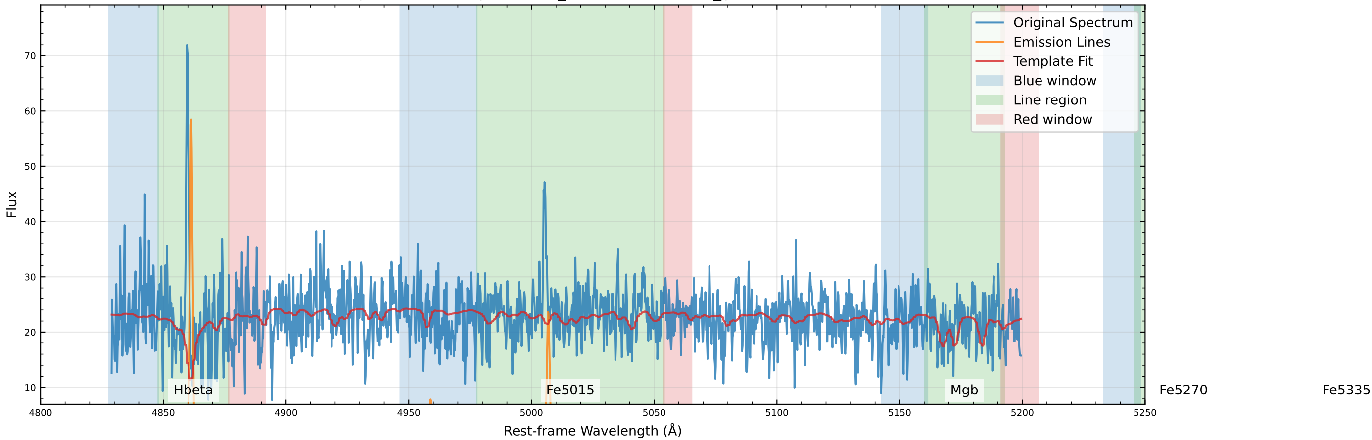
Original Data Comparison (v_star=-61.5 km/s, v_gas=-92.3 km/s)
