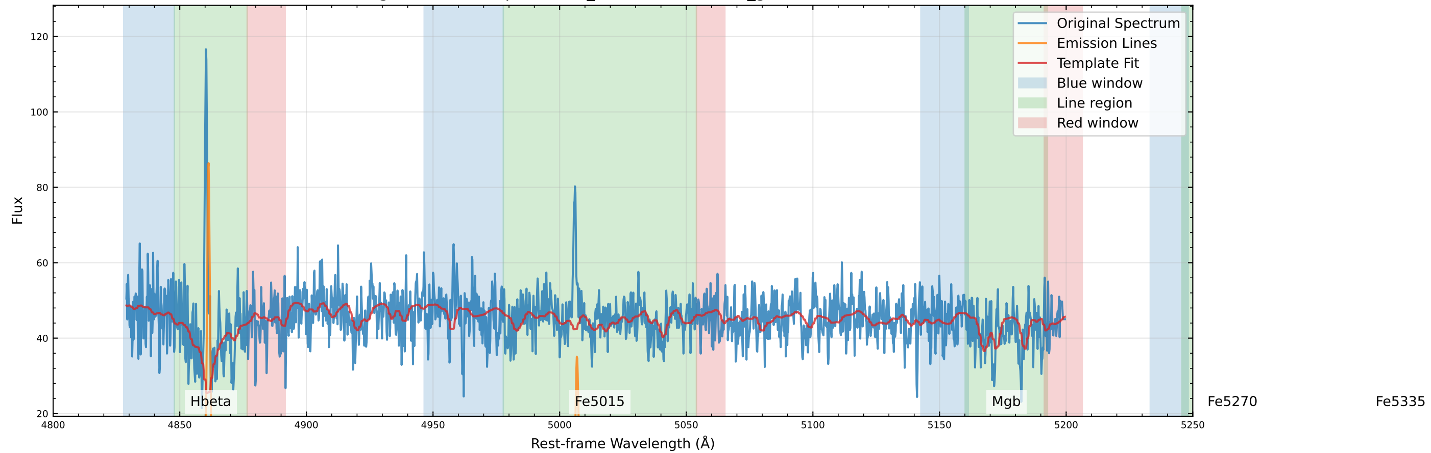
Original Data Comparison (v_star=-90.0 km/s, v_gas=-58.8 km/s)
