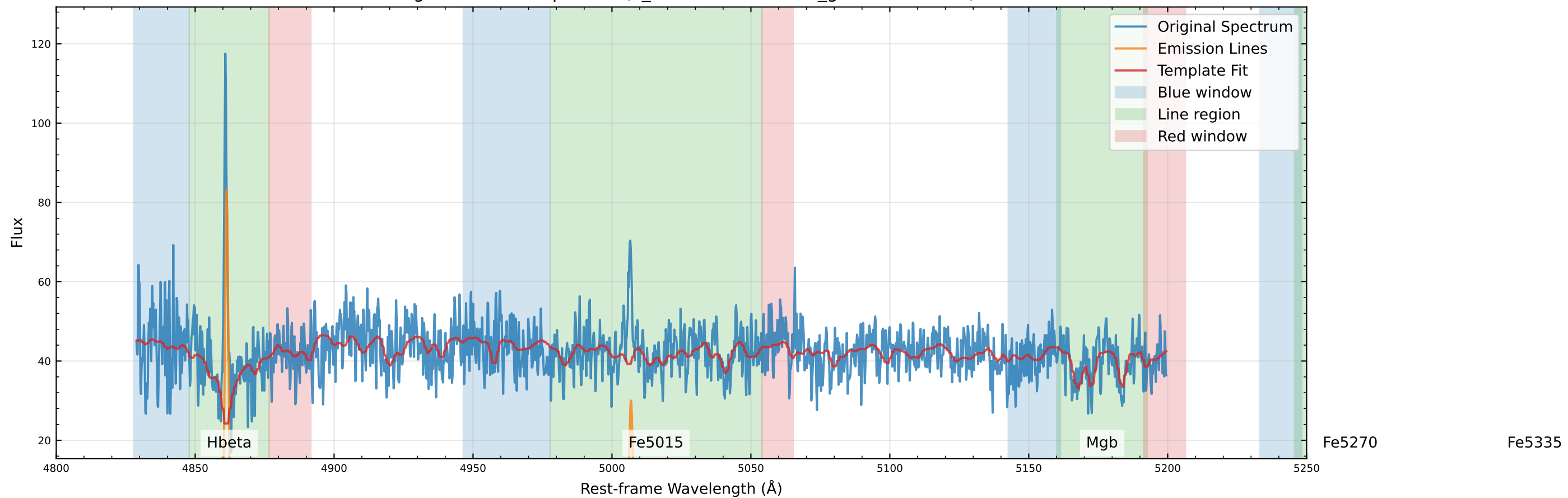
Original Data Comparison (v_star=-27.0 km/s, v_gas=-25.0 km/s)
