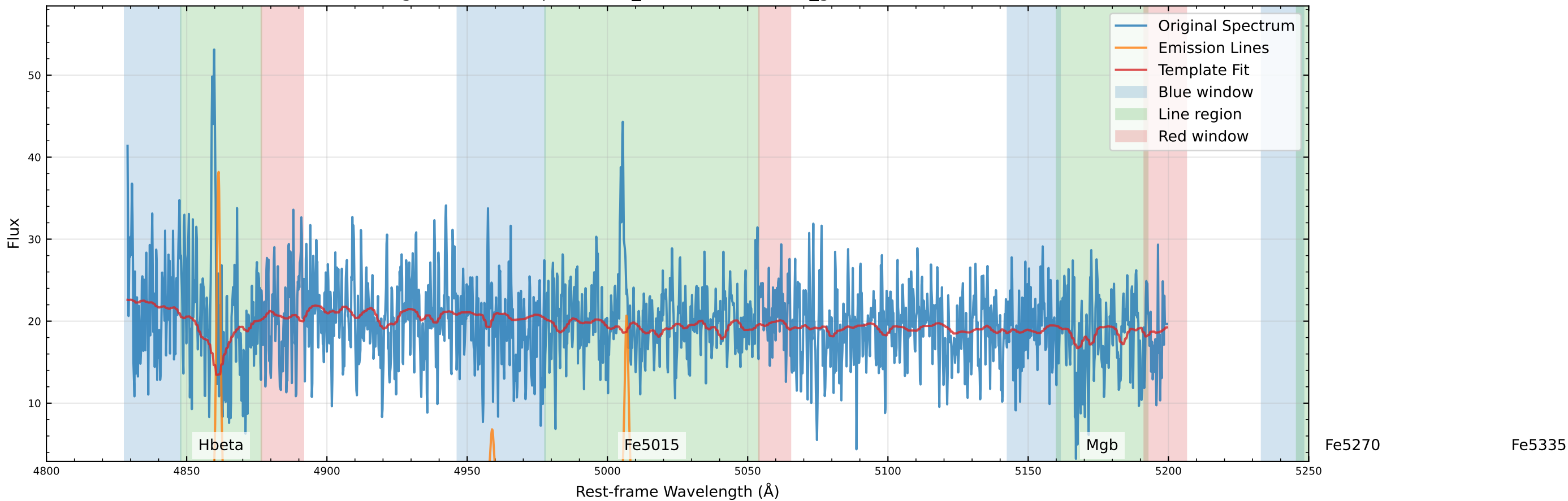
Original Data Comparison (v_star=-88.9 km/s, v_gas=-105.2 km/s)
