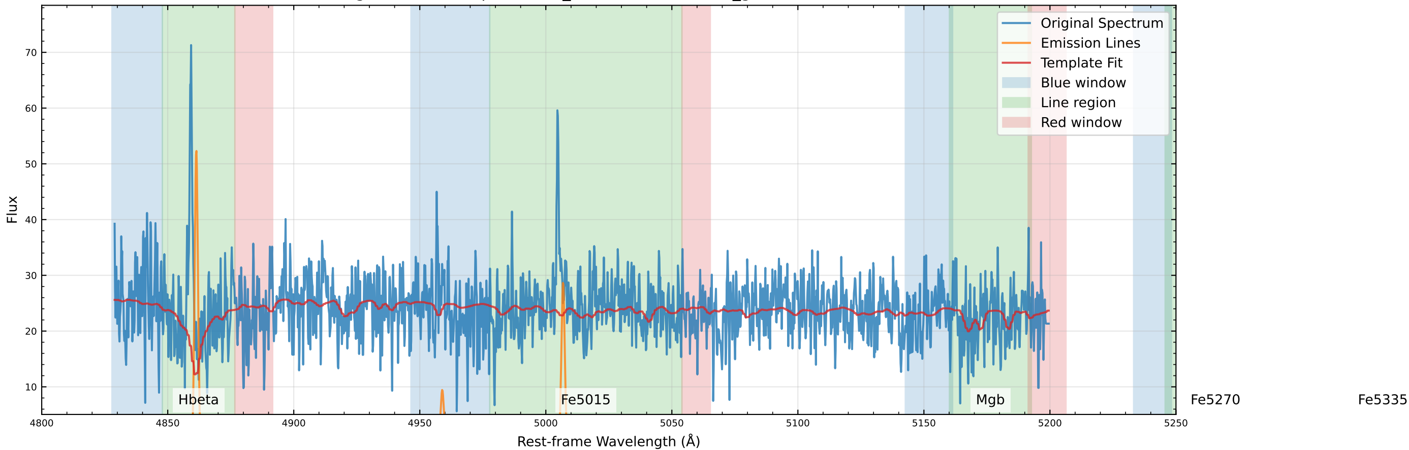
Original Data Comparison (v_star=-127.6 km/s, v_gas=-129.3 km/s)
