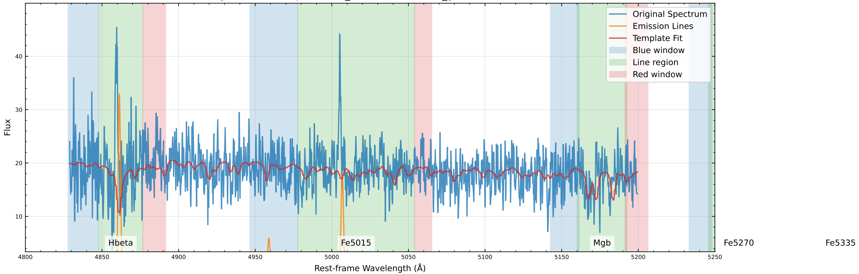
Original Data Comparison (v_star=-94.1 km/s, v_gas=-109.5 km/s)
