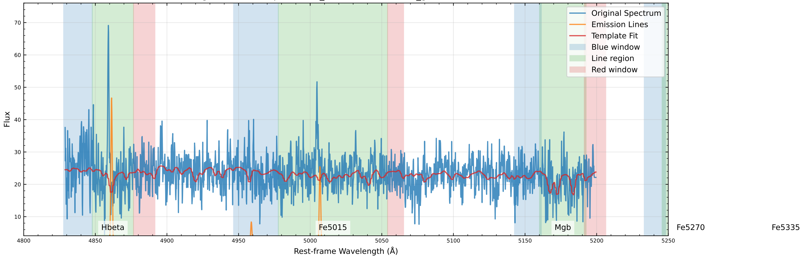
Original Data Comparison (v_star=-129.1 km/s, v_gas=-135.3 km/s)
