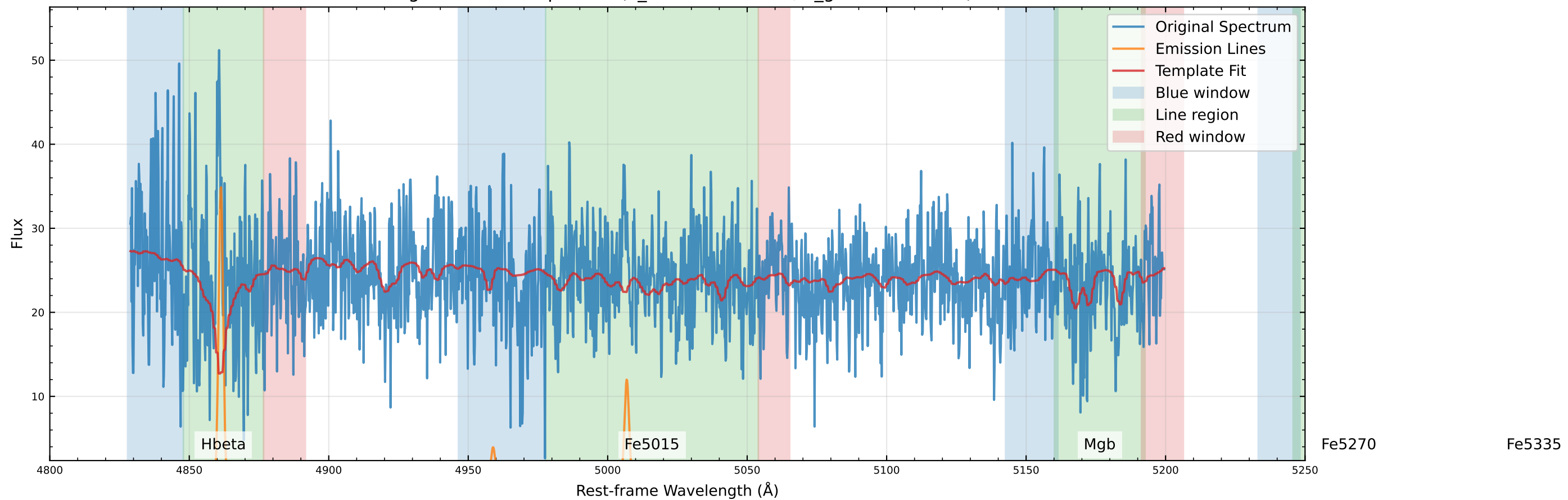
Original Data Comparison (v_star=-65.6 km/s, v_gas=-49.2 km/s)
