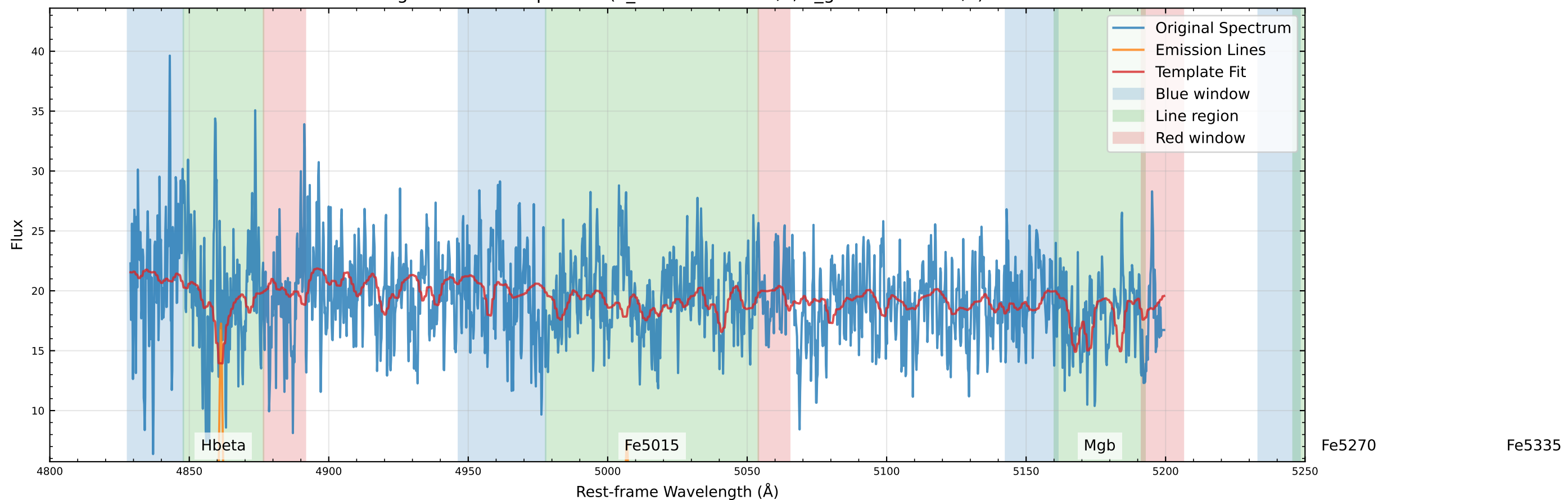
Original Data Comparison (v_star=-152.0 km/s, v_gas=-126.0 km/s)
