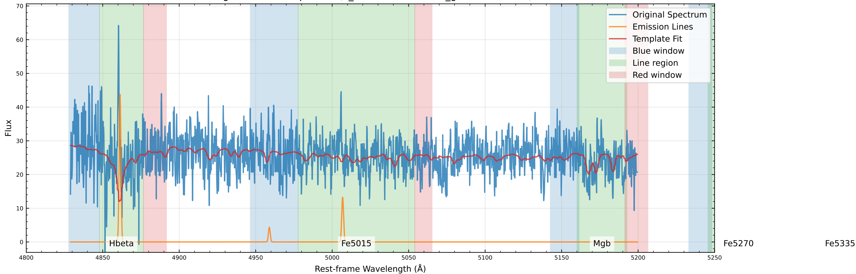
Original Data Comparison (v_star=-84.7 km/s, v_gas=-65.7 km/s)
