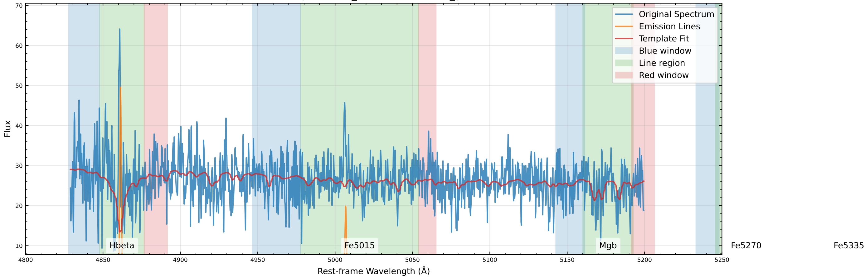
Original Data Comparison (v_star=-51.6 km/s, v_gas=-44.3 km/s)
