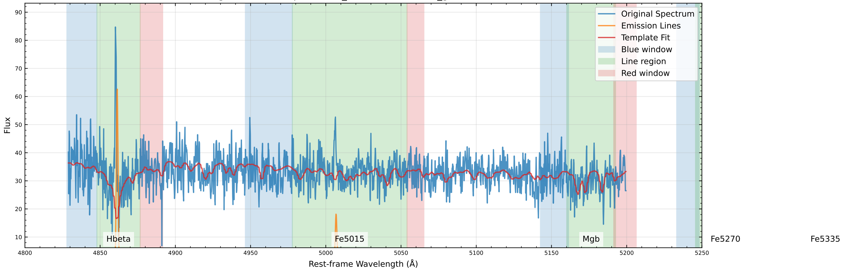
Original Data Comparison (v_star=-45.5 km/s, v_gas=-60.0 km/s)
