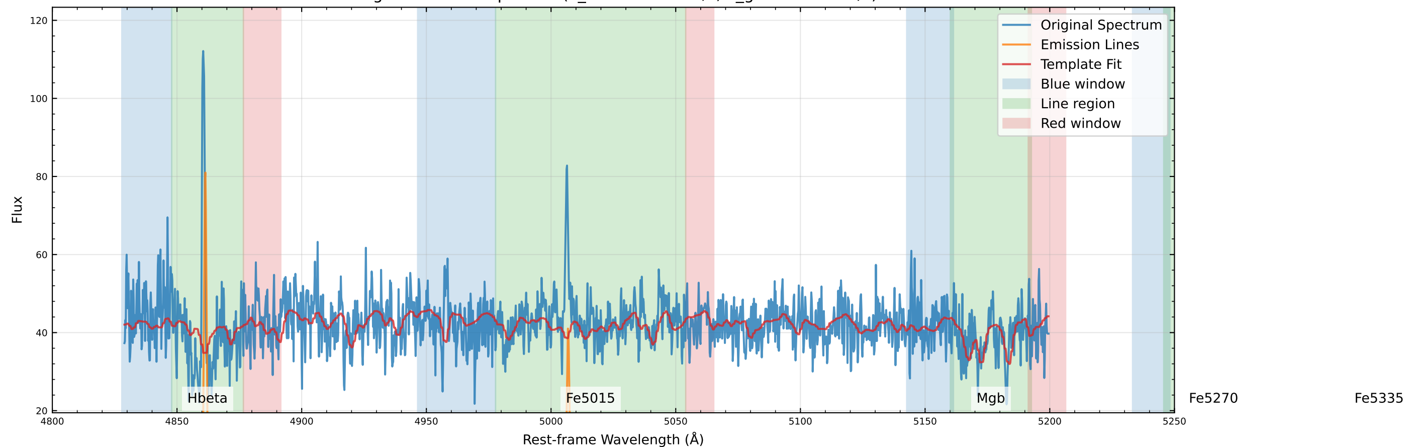
Original Data Comparison (v_star=-64.9 km/s, v_gas=-45.1 km/s)
