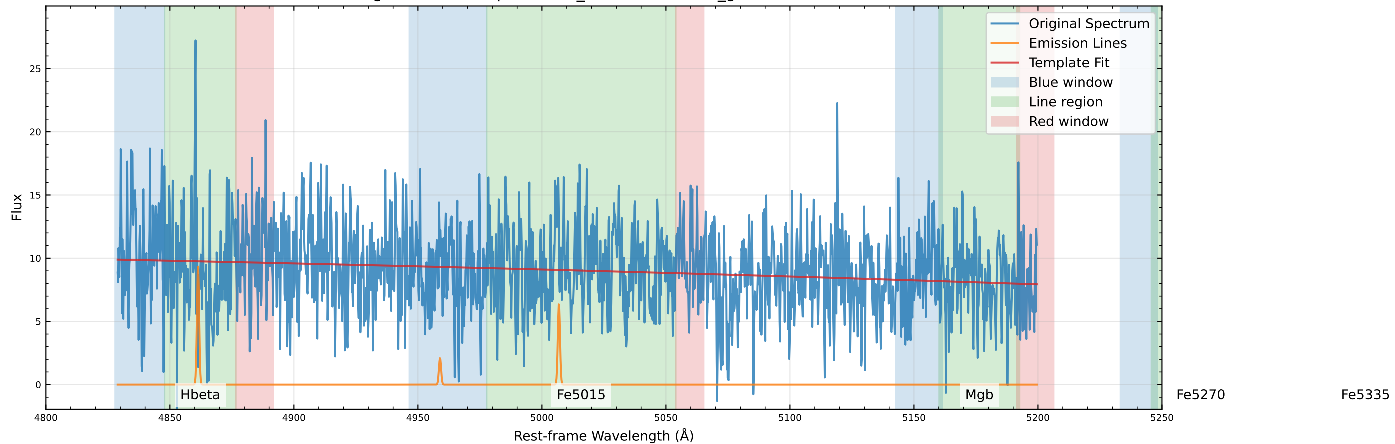
Original Data Comparison (v_star=0.0 km/s, v_gas=-68.9 km/s)
