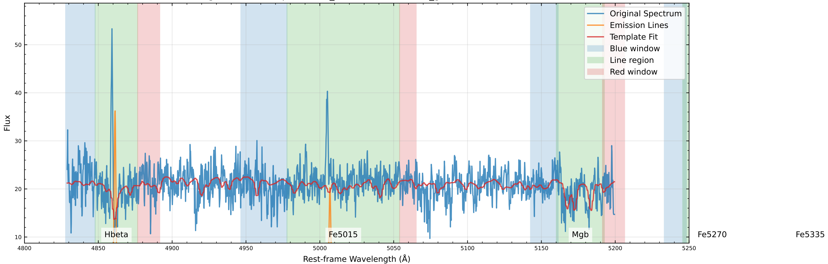
Original Data Comparison (v_star=-108.5 km/s, v_gas=-127.4 km/s)
