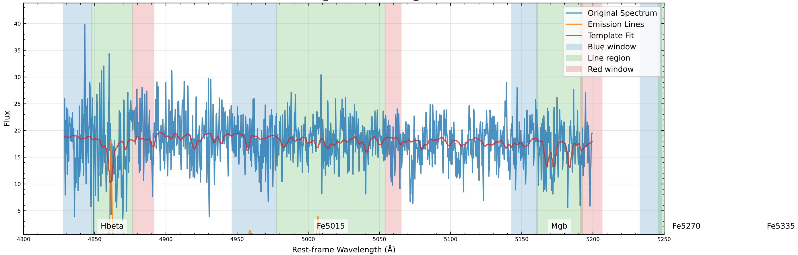
Original Data Comparison (v_star=-72.5 km/s, v_gas=-73.0 km/s)
