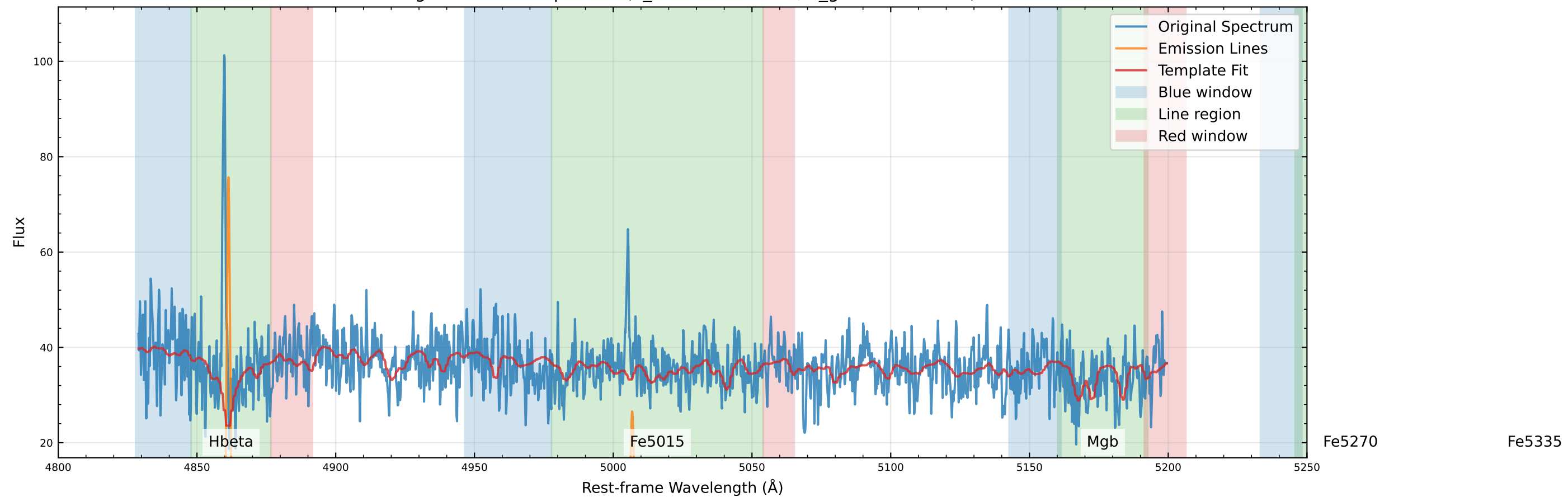
Original Data Comparison (v_star=-95.8 km/s, v_gas=-97.5 km/s)
