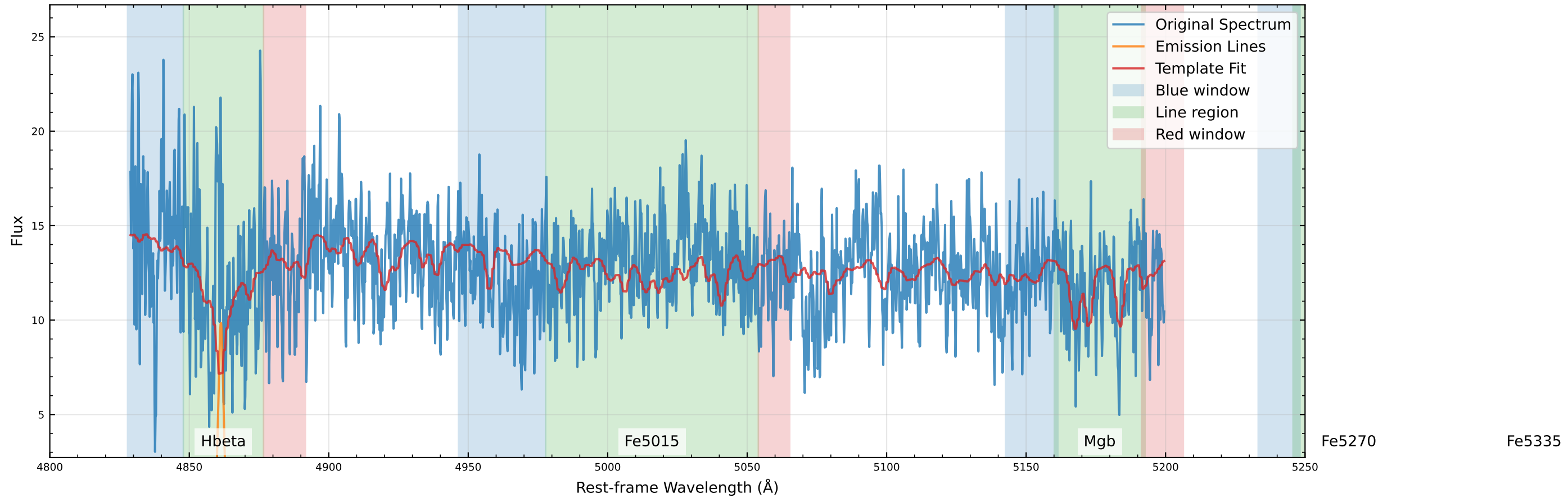
Original Data Comparison (v_star=-44.3 km/s, v_gas=-54.7 km/s)
