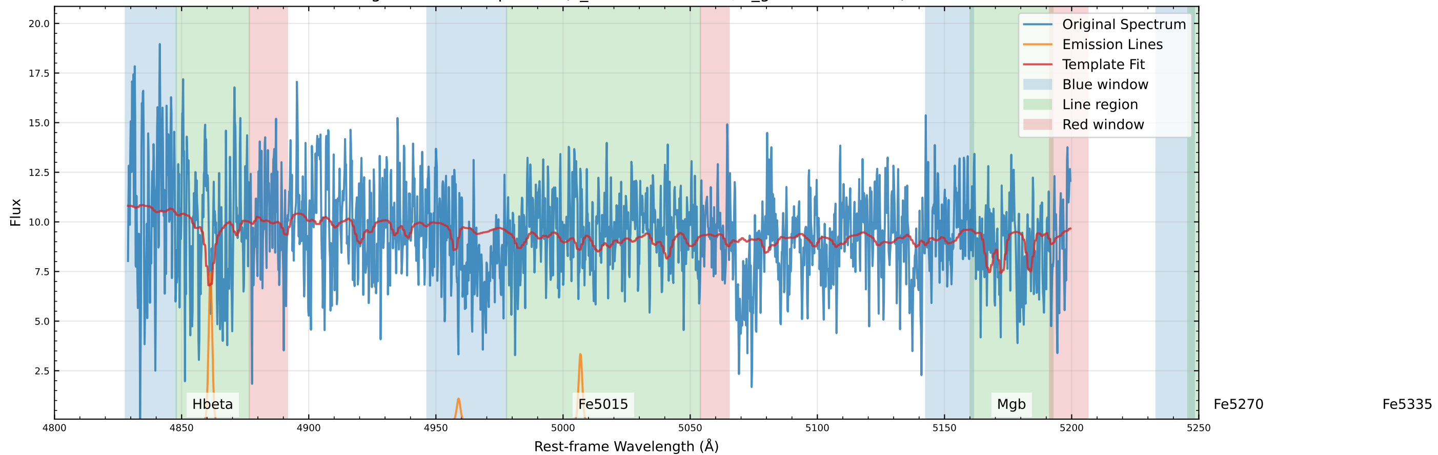
Original Data Comparison (v_star=-133.4 km/s, v_gas=-125.5 km/s)
