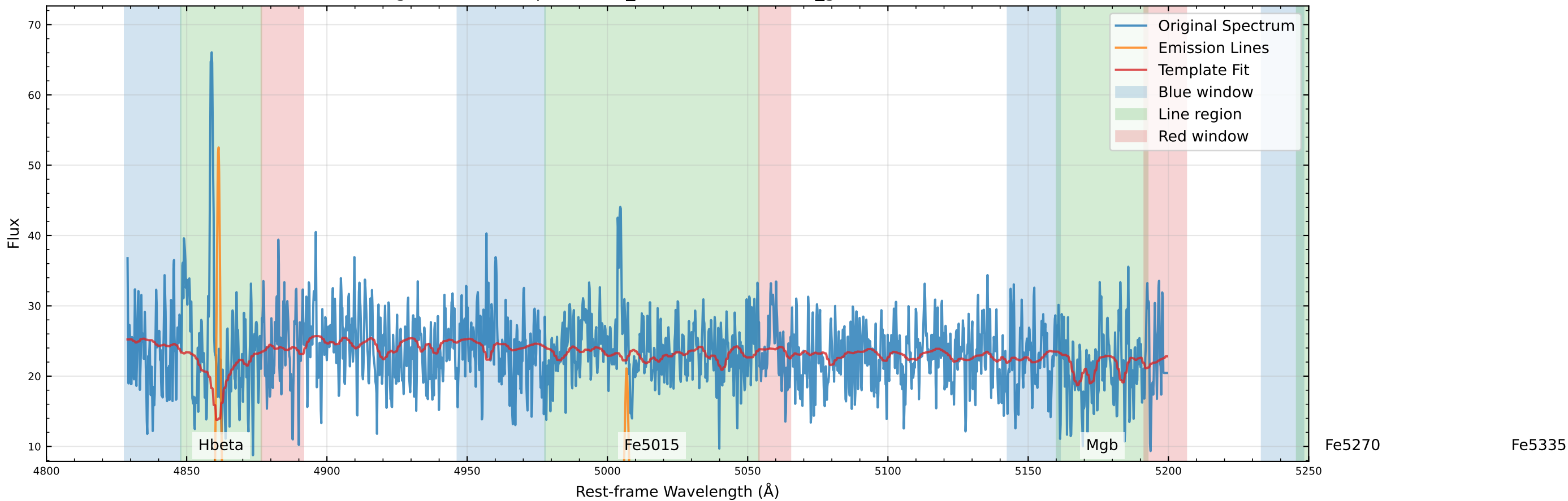
Original Data Comparison (v_star=-137.8 km/s, v_gas=-150.9 km/s)
