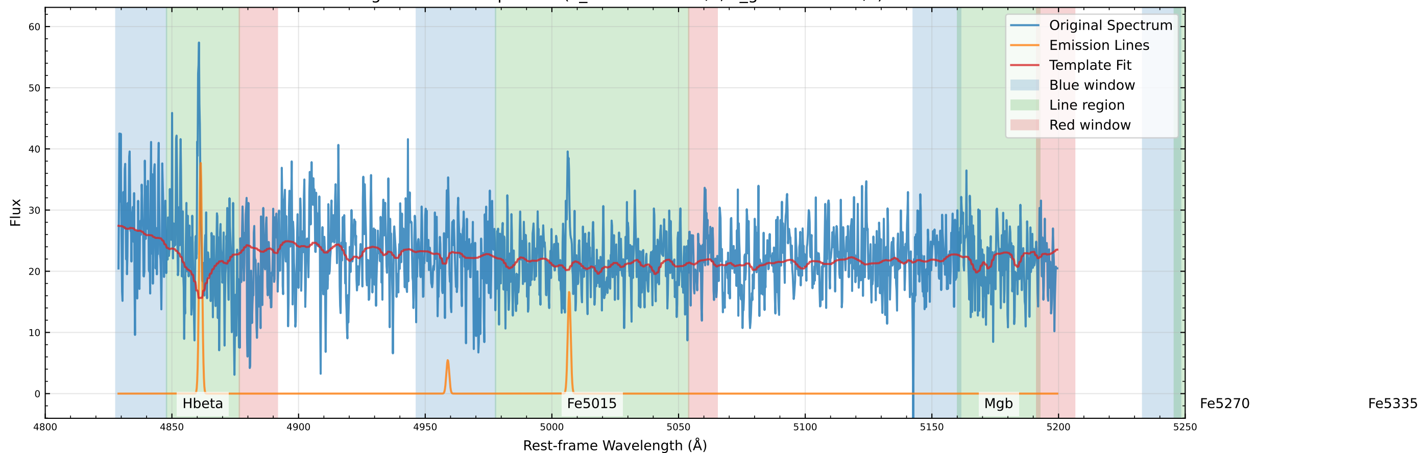
Original Data Comparison (v_star=-43.9 km/s, v_gas=-40.4 km/s)
