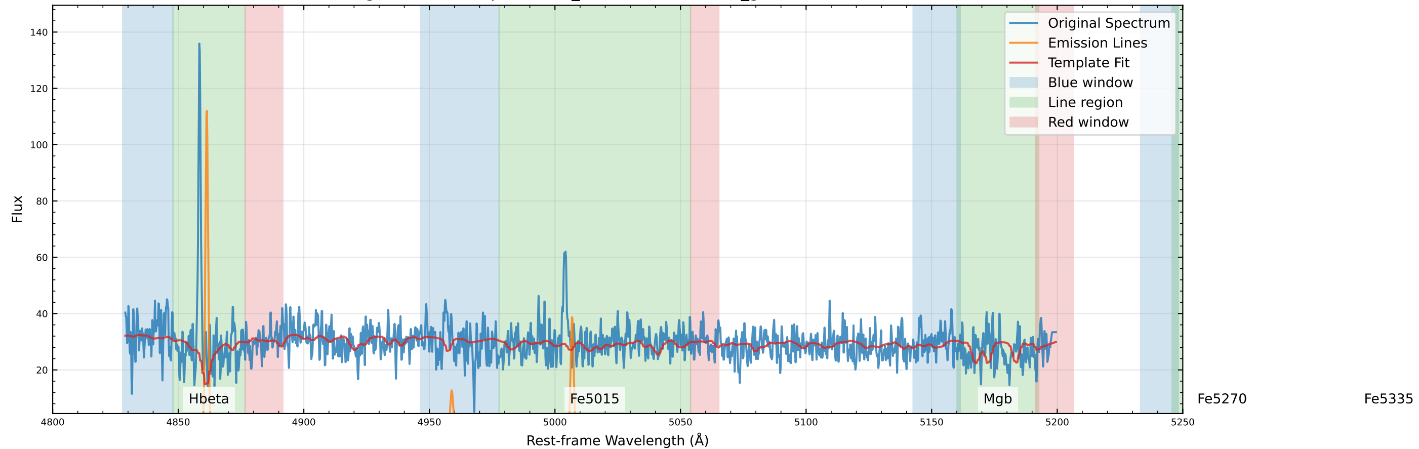
Original Data Comparison (v_star=-172.0 km/s, v_gas=-175.8 km/s)
