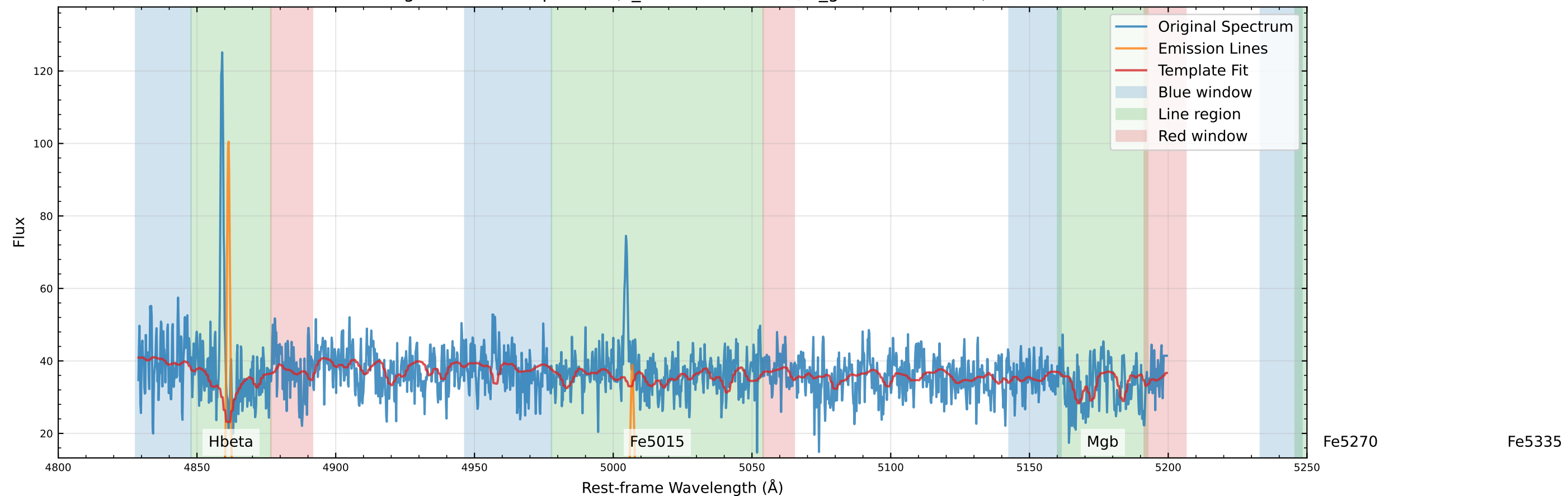
Original Data Comparison (v_star=-133.2 km/s, v_gas=-141.0 km/s)
