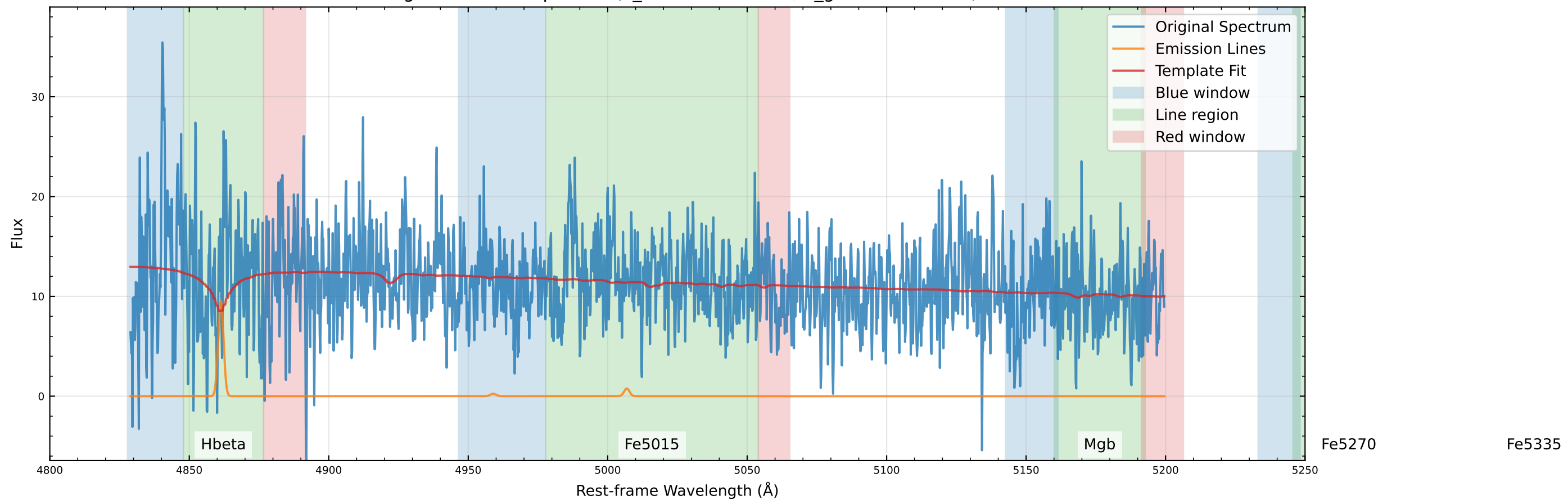
Original Data Comparison (v_star=114.9 km/s, v_gas=104.6 km/s)
