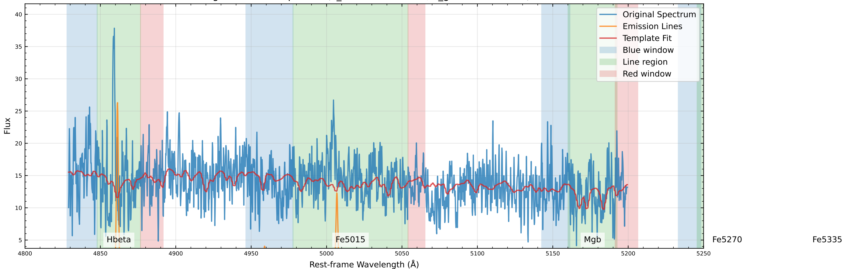
Original Data Comparison (v_star=-122.6 km/s, v_gas=-146.4 km/s)
