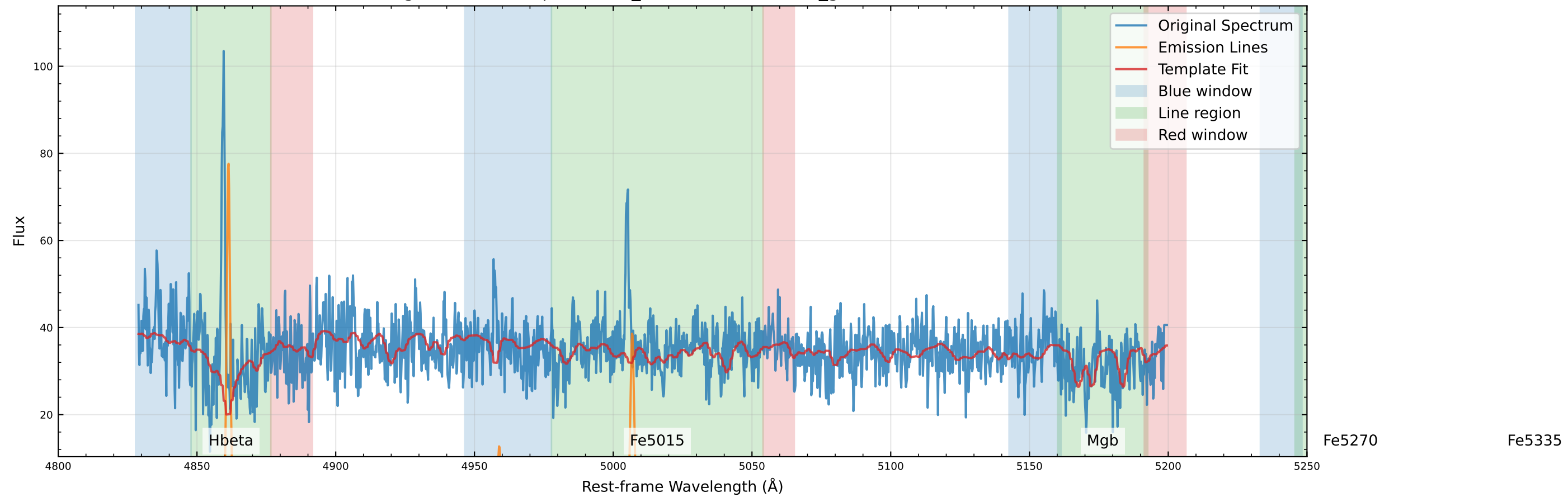
Original Data Comparison (v_star=-108.9 km/s, v_gas=-114.1 km/s)
