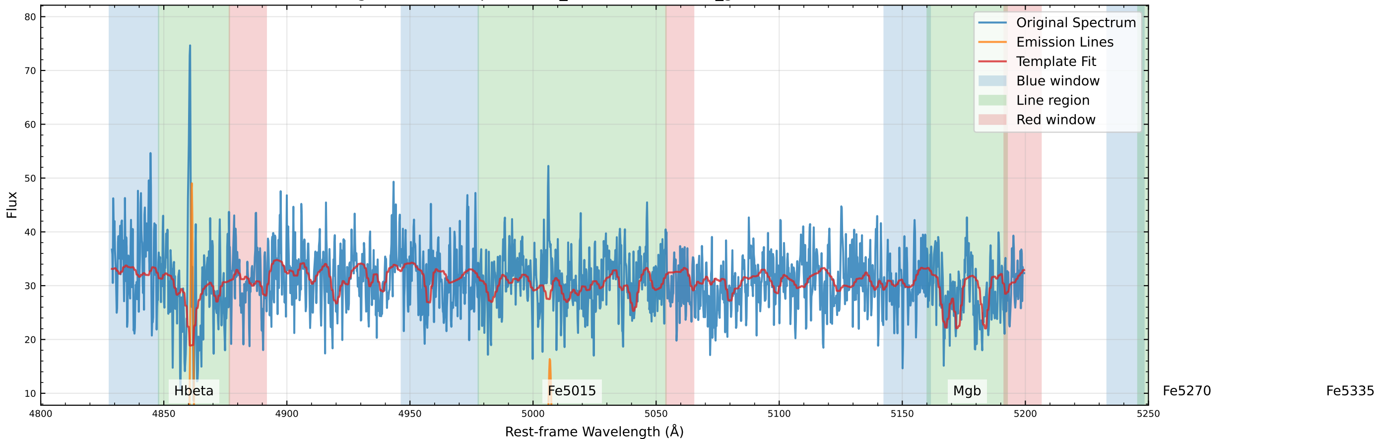
Original Data Comparison (v_star=-45.7 km/s, v_gas=-53.0 km/s)
