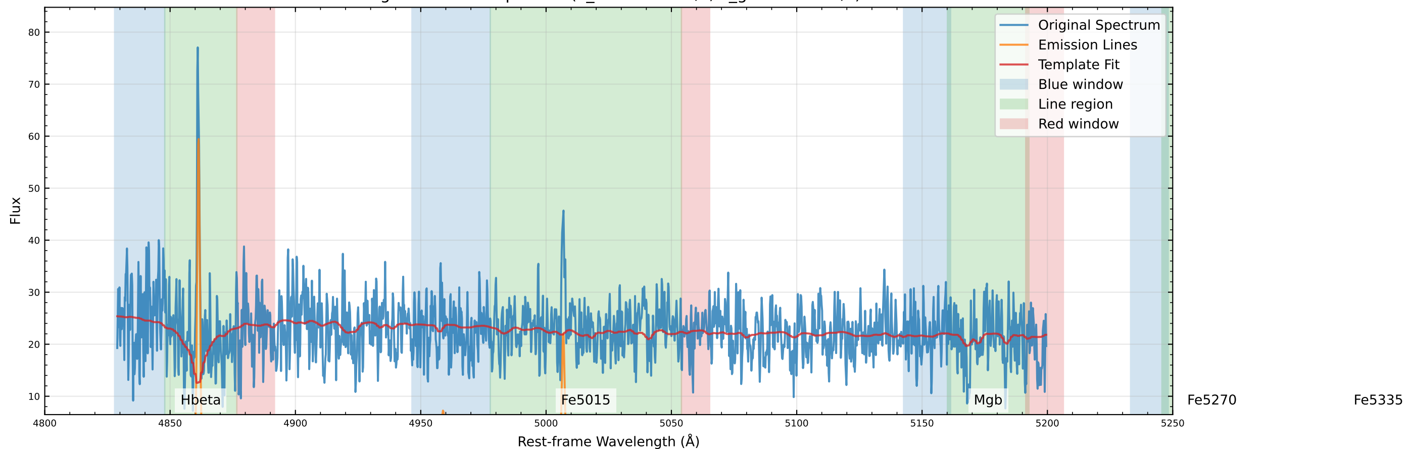
Original Data Comparison (v_star=7.7 km/s, v_gas=-8.9 km/s)
