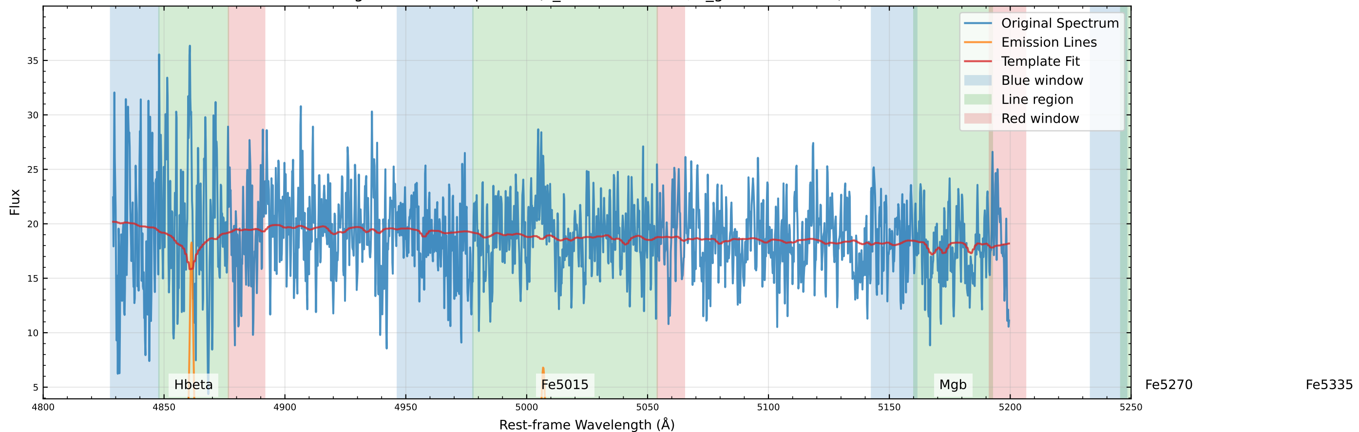
Original Data Comparison (v_star=-27.2 km/s, v_gas=-44.1 km/s)
