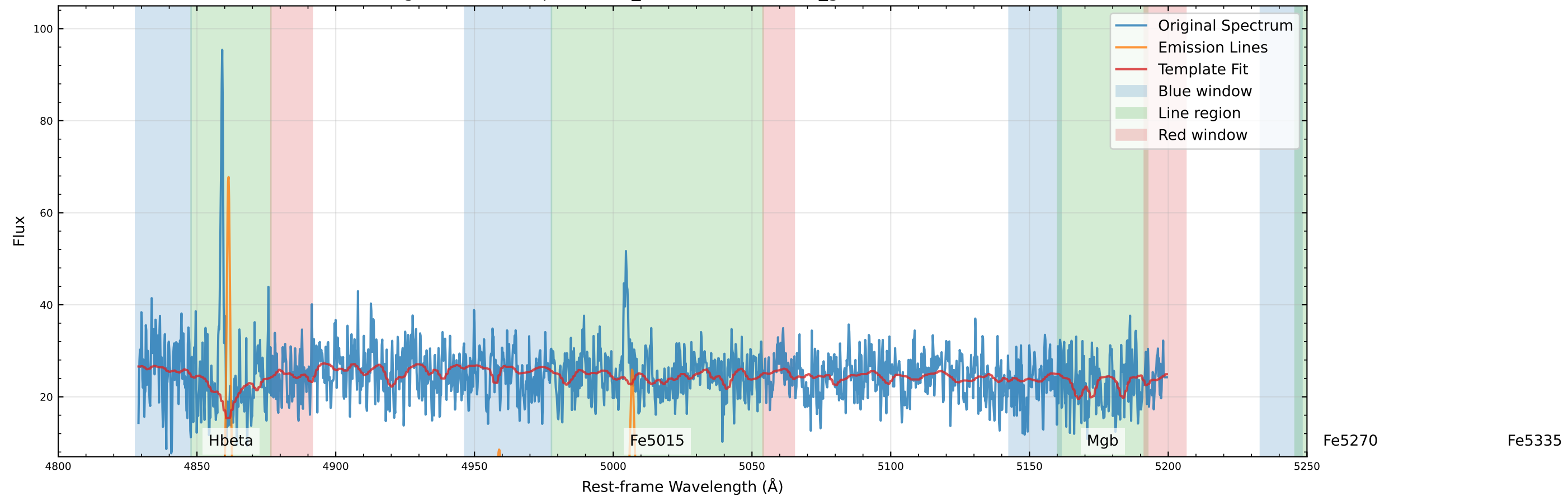
Original Data Comparison (v_star=-112.2 km/s, v_gas=-143.8 km/s)
