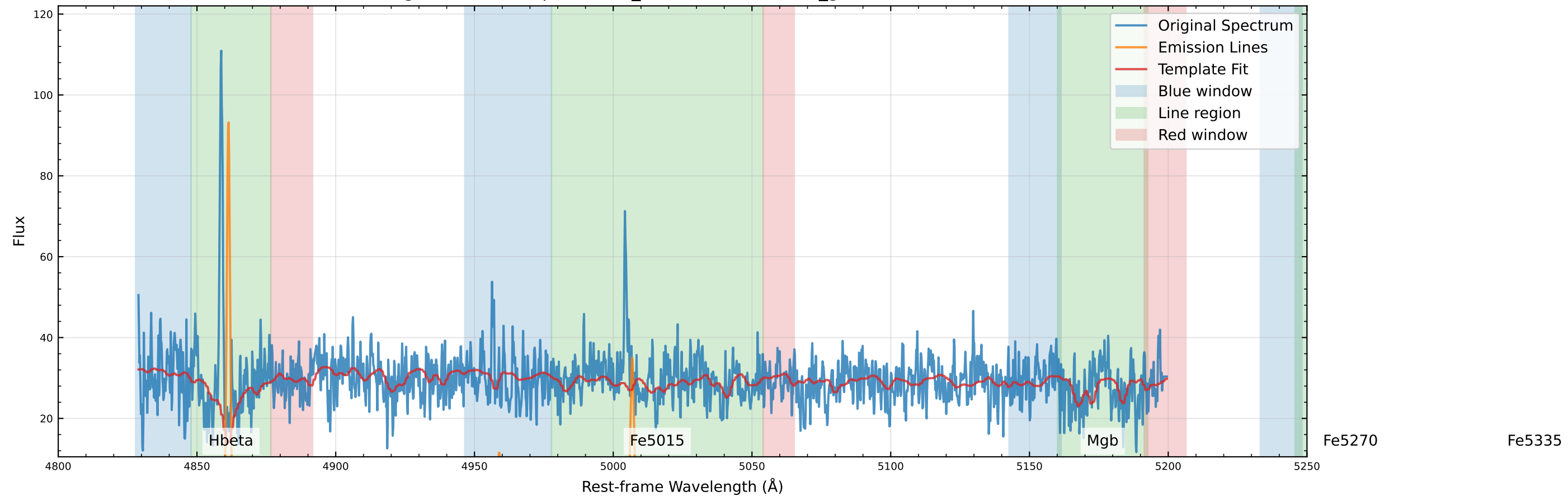
Original Data Comparison (v_star=-148.7 km/s, v_gas=-157.5 km/s)
