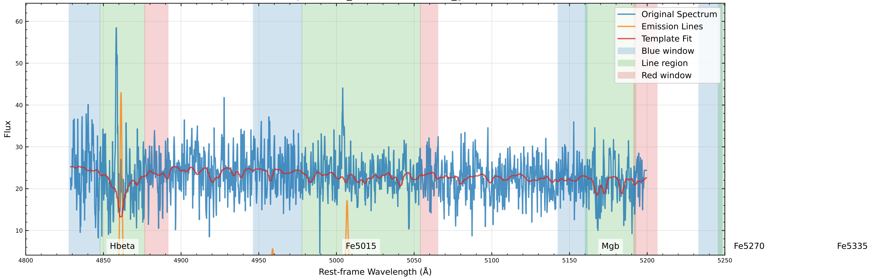
Original Data Comparison (v_star=-138.2 km/s, v_gas=-176.1 km/s)
